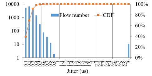
(c) Jitter distribution among all flows.
