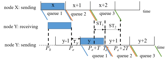
Fig. 3. Cyclic queue scheduling on core LDN nodes.
