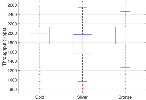
Figure 7: sLB and FIFO throughput results. Removal of SQ removes any aspect of intelligent queuing causing significant violations in gold flow throughput requirements.
