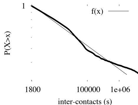
Figure 5: Log-log plot of the CCDF of aggregate inter-contacts in Dartmouth.
